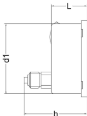
type D (Ø 63 mm, without blow-out back)
