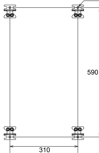
<-W (Wall mount) dimension> 4-M8 or \phi 10
