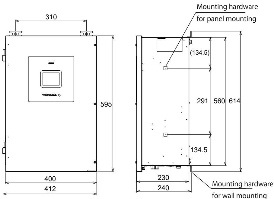
<-W (Wall mount) dimension> 4-M8 or \phi 10
