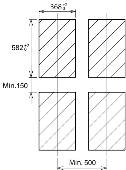
<-P (Panel mount) Panel cut dimension>
