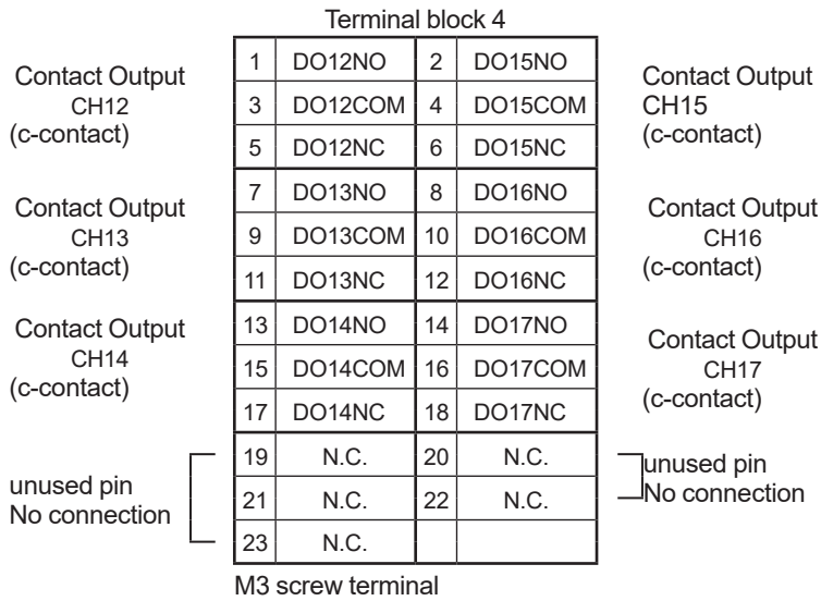
Figure 2.18 Terminal block 4: Contact output (c-contact)
