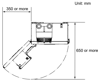
Figure 2.1 Maintenance space
