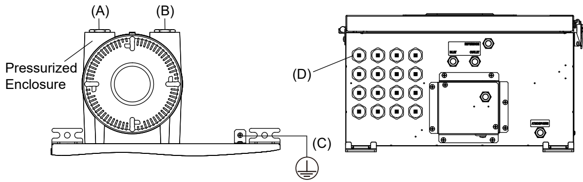
Figure 2.5 Cable position
