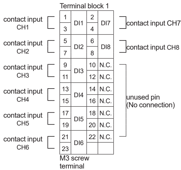
Figure 2.15 Terminal block 1: Contact input terminal
