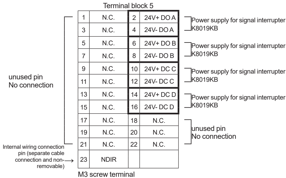
Figure 2.20 Terminal block 5: Power supply for signal interrupter
