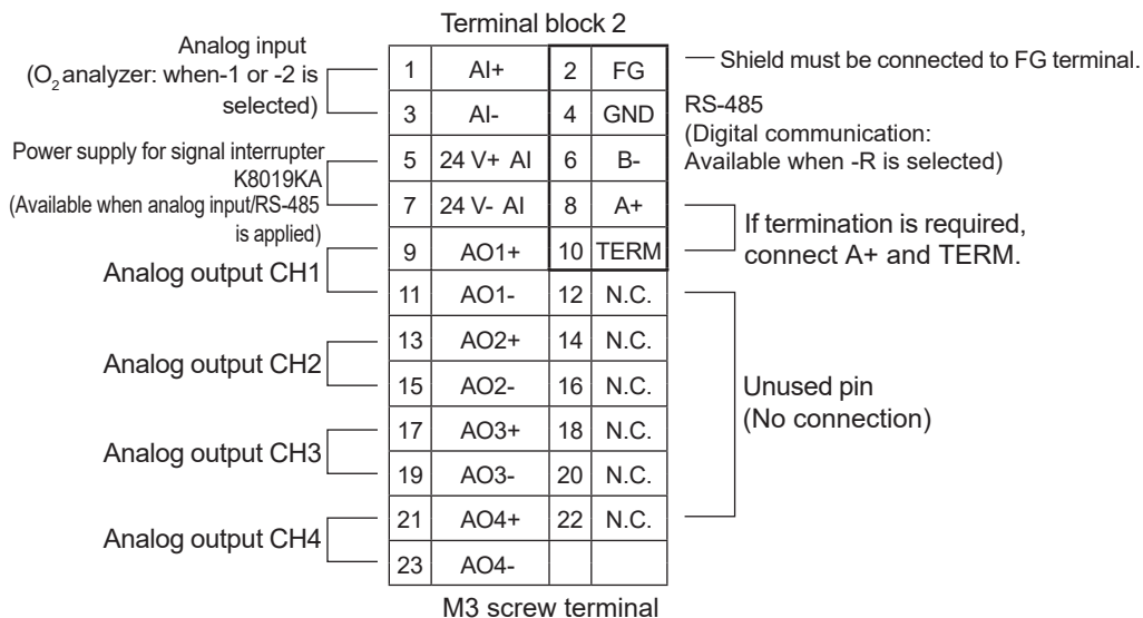
Figure 2.16 Terminal block 2: analog input/analog output/RS-485
