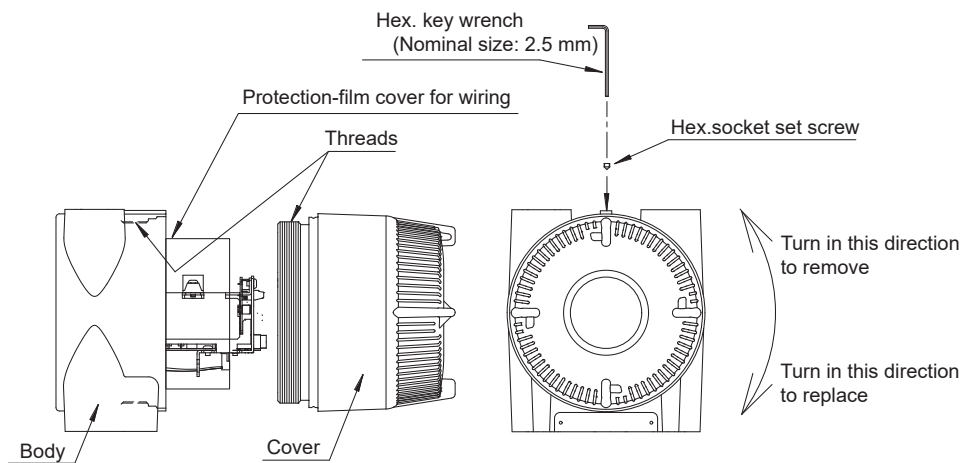
Figure 2.12 Opening/closing the cover of the protection system
