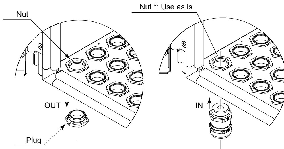
Figure 2.11 IR810S I/O (or signal) cable gland installation
