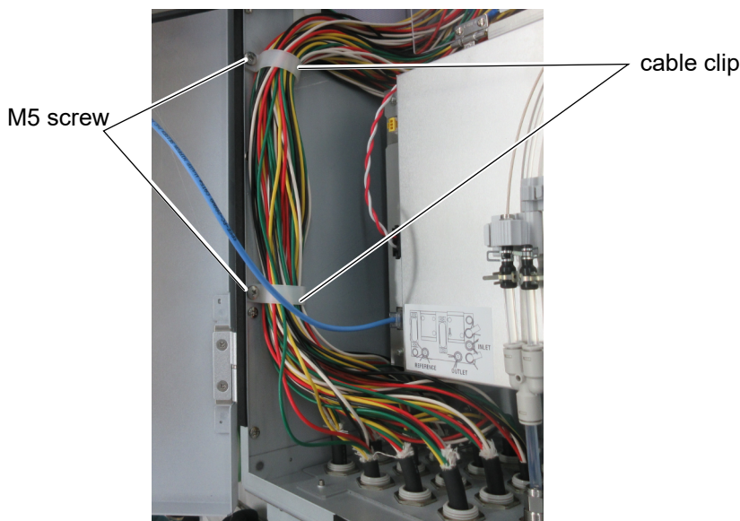
Route the cable from the left side. After wiring, fasten the cable with the supplied cable clip and M5 screws. The tightening torque is 2.0 N·m.
