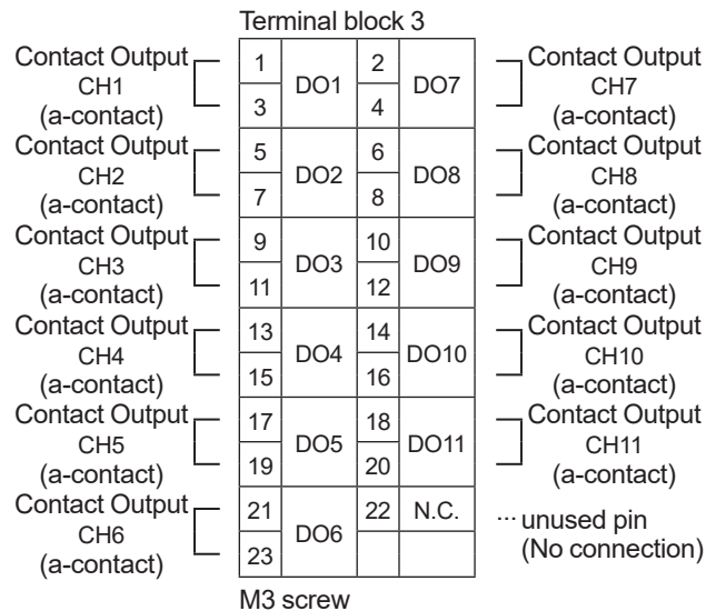
Figure 2.17 Terminal block 3: Contact output (a-contact)
