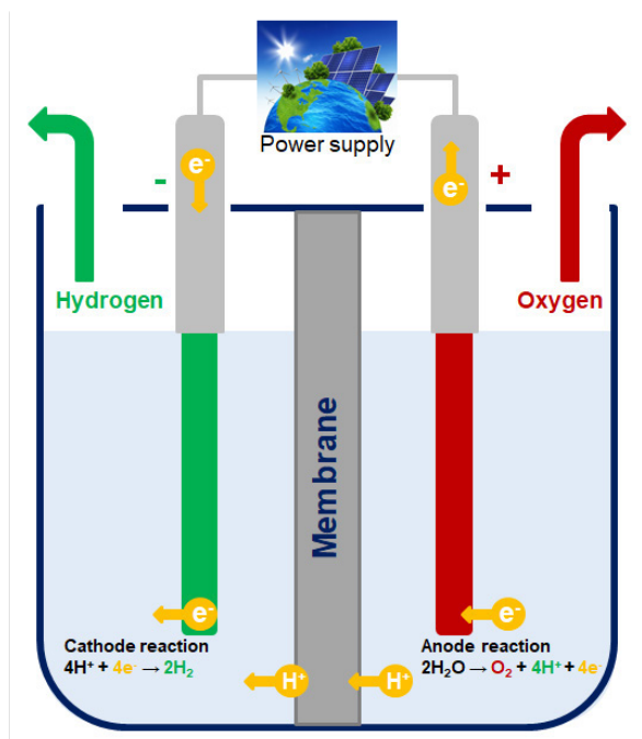
Figure 1: Typical polymer electrolyte membrane cell.
