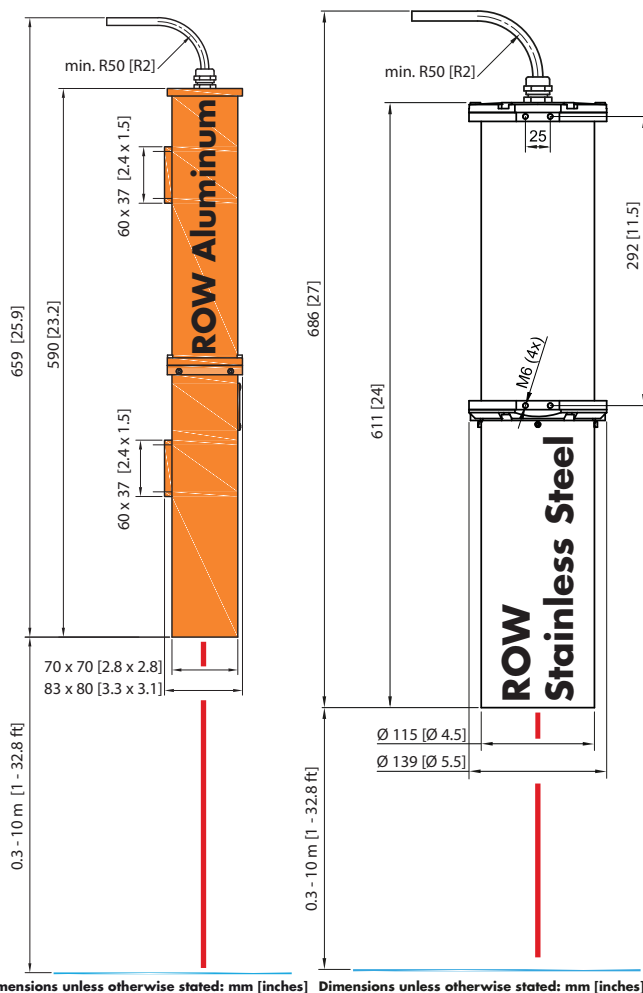
Dimensions unless otherwise stated: mm [inches]
