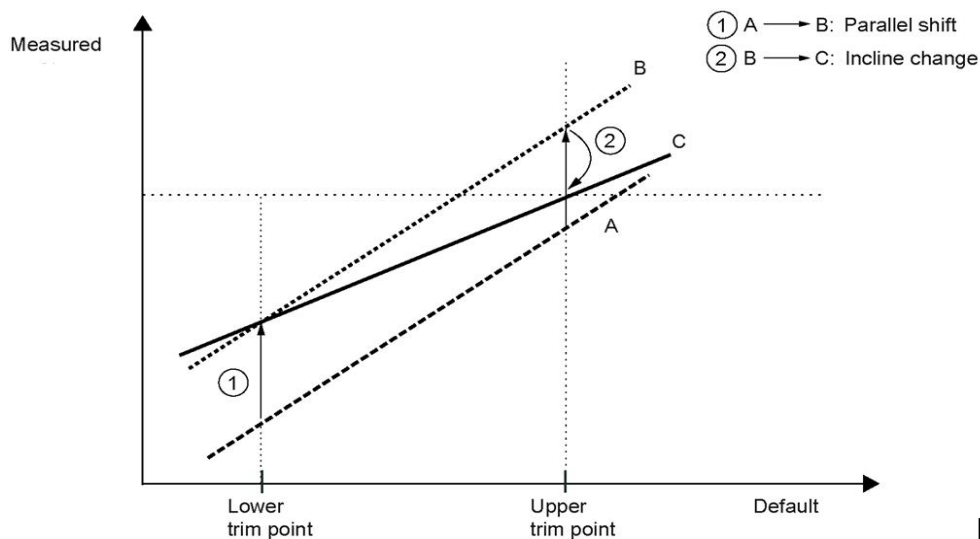
Figure 3: Sensor Trim
