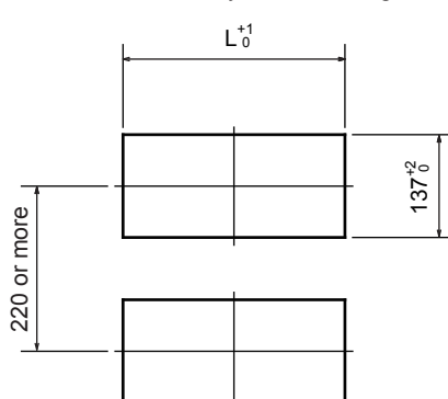
Pane Cutout Dimensions
